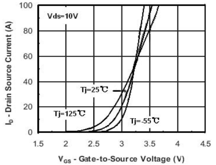
Transfer Characteristic
