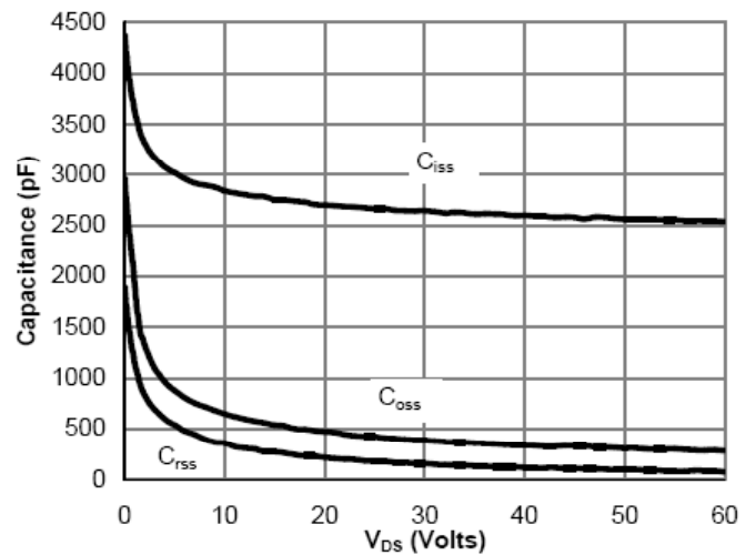
Capacitance
